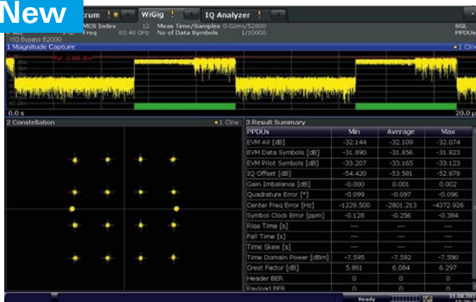
Analysis of a WLAN 802.11ad signal at 60.48 GHz with a 16QAM modulation and an EVM of -32 dB.
