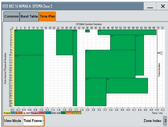
The signal generator graphically displays the configured WiMAX™ signal. The time plan shows the different WiMAX™ zones, segments and burst types.
