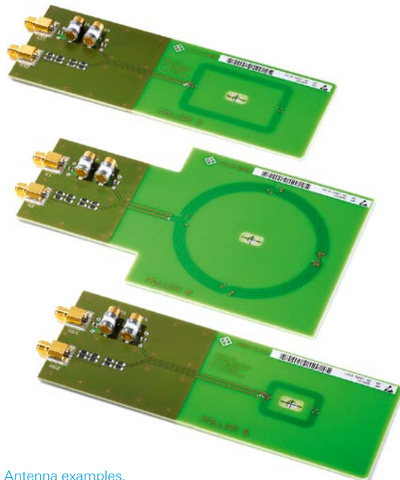
Antenna examples.
