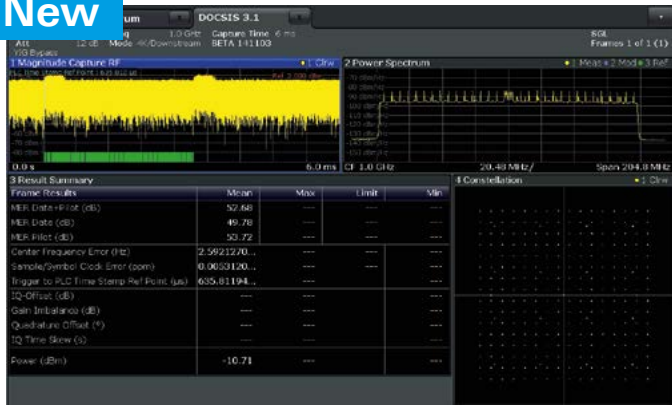
Analysis of DOCSIS 3.1 signal with R&S®FSW-K192 option.
