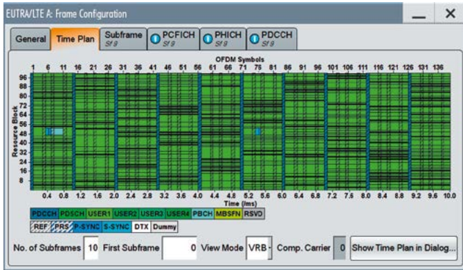
R&S®SMW-K55 LTE time plan example ( download ).
