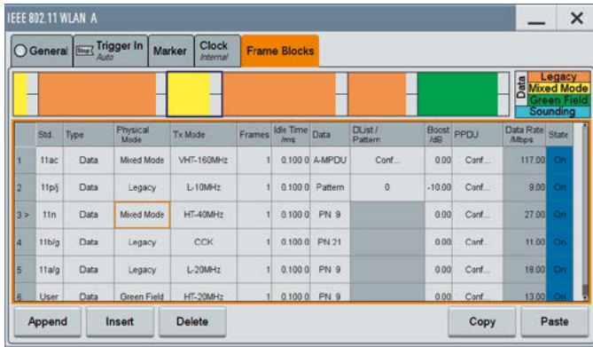
IEEE802.11 frameblock sequencer configuration menu of the R&S®SMW200A.
