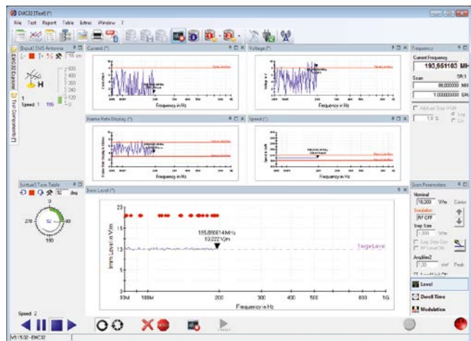
EMS qualification test with several EUT monitoring channels.
