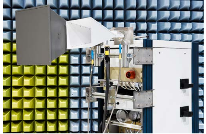
EMS microwave test.
