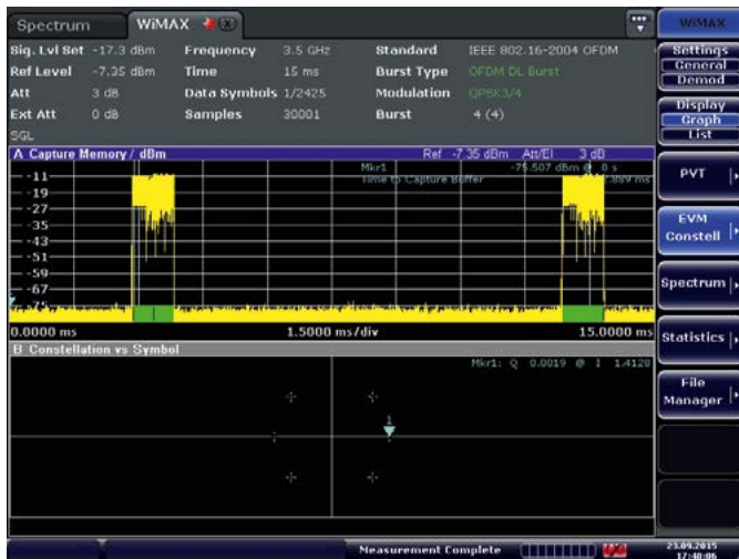
Demodulation of a WiMAX™ signal with R&S®FSV-K93.
