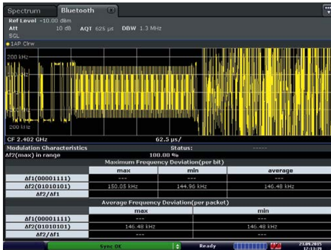
Analysis of a Bluetooth® signal with R&S®FSV-K8.
